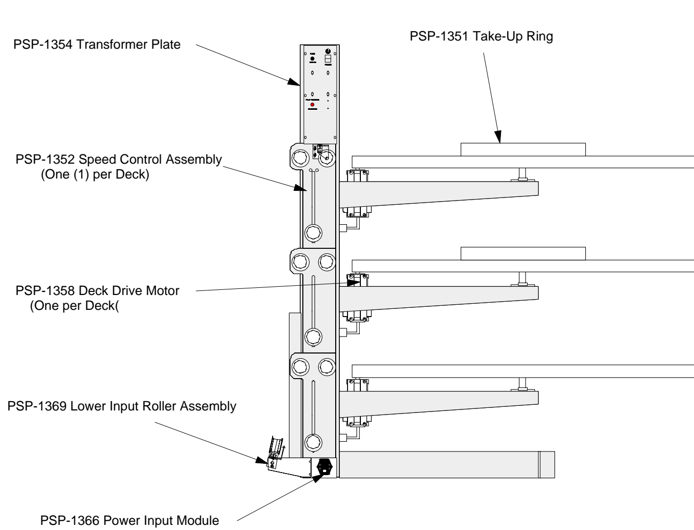
TAKE-UP SIDE AND REPLACEMENT ASSEMBLIES
