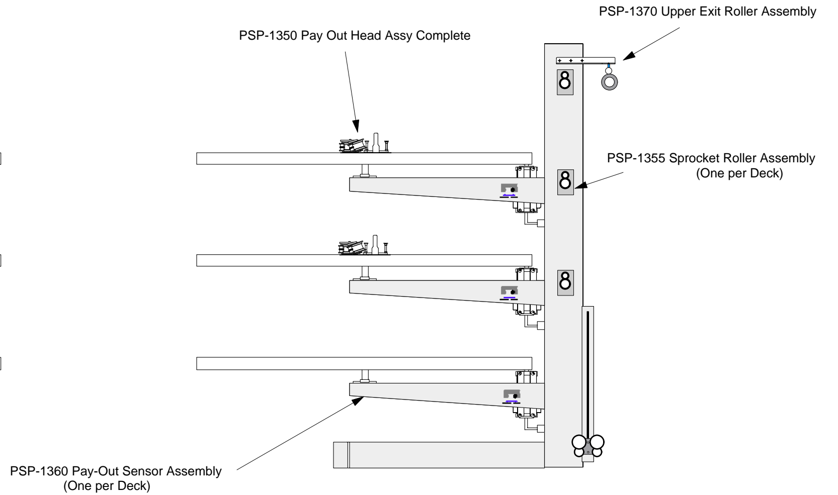
PAY-OUT SIDE AND REPLACEMENT ASSEMBLIES
